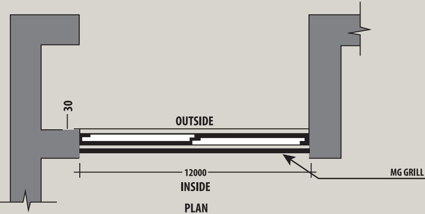
W1 2.5 TRACKS ALUMINIUM SLIDING WINDOW WITH FIXED GLASS PANEL AS PER DETAIL. 2 GLAZED AND BUG MESH PANEL, WITH LOCKING ARRANGEMENT. GLAZING THICKNESS TO BE CONFIRMED AS PER WIND LOAD FACTOR.
