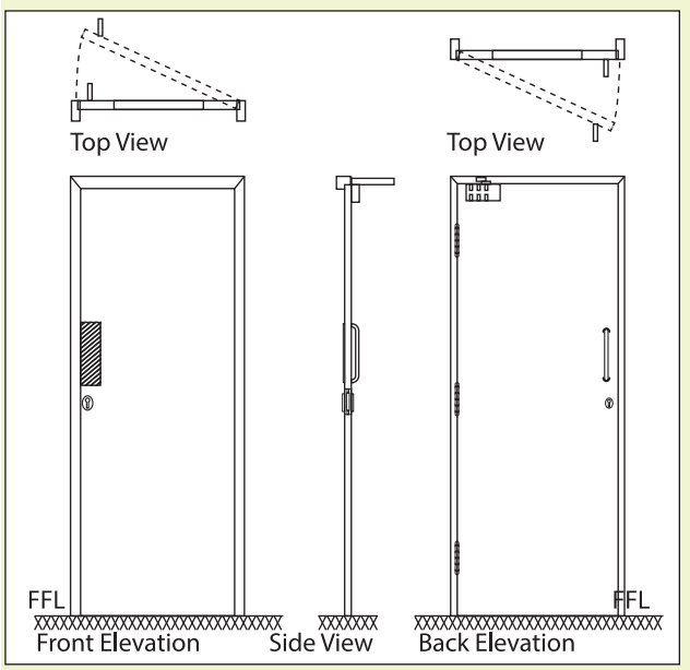
Single Leaf Solid Door
