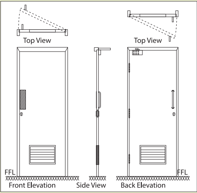
Single Leaf Door with Full Louver
