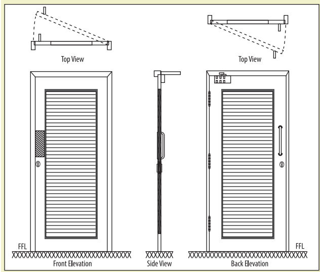
Single Leaf Door with Full Louver
